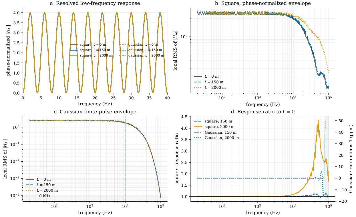
Figure 3. Atomic transfer functions under Model A. (a) All six low-frequency curves are drawn; coincident lines reflect equal responses rather than omitted data. (b) Square-pulse propagation changes the finite-pulse envelope, strongly for 2000 m. (c) All Gaussian magnitudes overlap because area compensation restores the Gaussian shape. (d) The left axis shows the positive square response ratio to L = 0 ; the right axis shows the Gaussian ratio offset in parts per million. Gaussian ratios are hidden once the L = 0 absolute RMS falls below 10^{-3} , where division by a vanishing response exaggerates truncation and numerical residuals.
