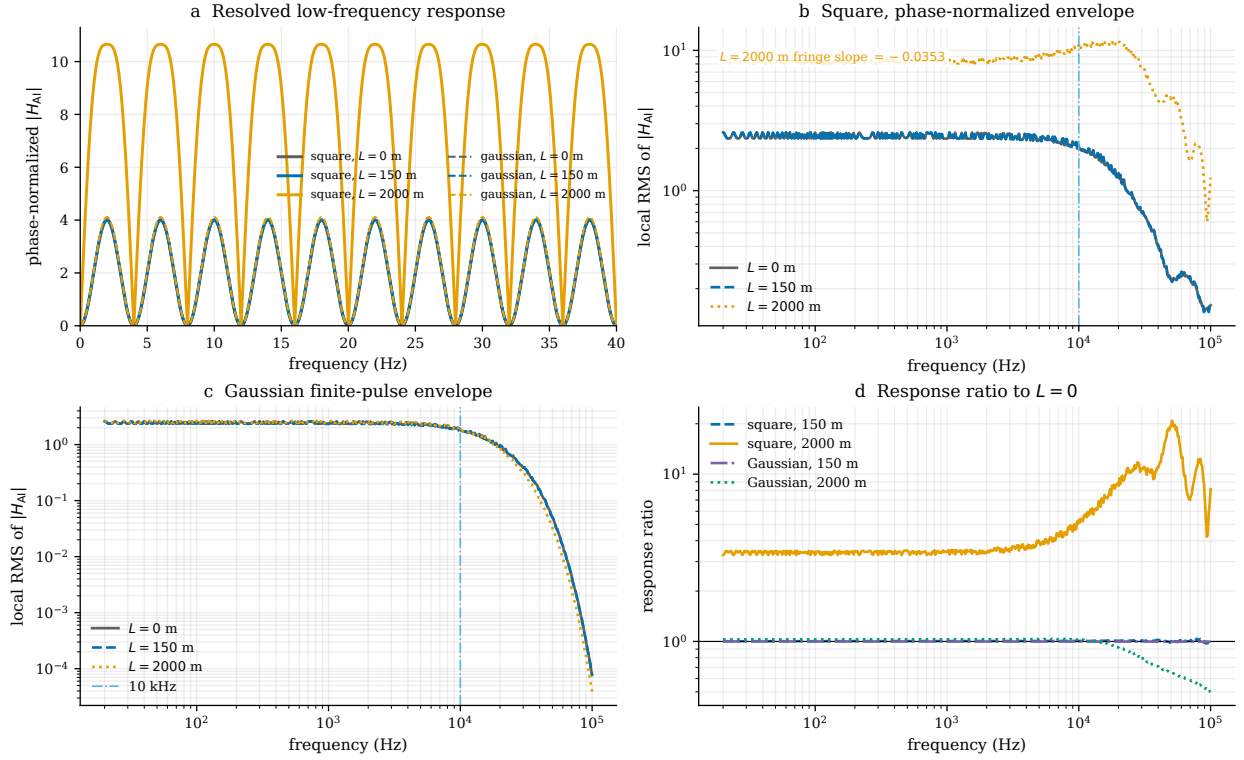
Figure 6. Atomic transfer functions under Model B. (a) All square and Gaussian distances are drawn and the vertical range is determined from the data, so the 2000 m square curve is no longer clipped. Coincident curves remain visible through distinct solid/dashed styles. (b) The square response is phase-normalized by the output-fringe slope; the annotation identifies the small 2000 m slope responsible for its large value. (c) Gaussian finite-pulse envelopes. (d) Positive ratios R_L/R_0 replace signed relative changes: values above one indicate amplification and values below one attenuation.
